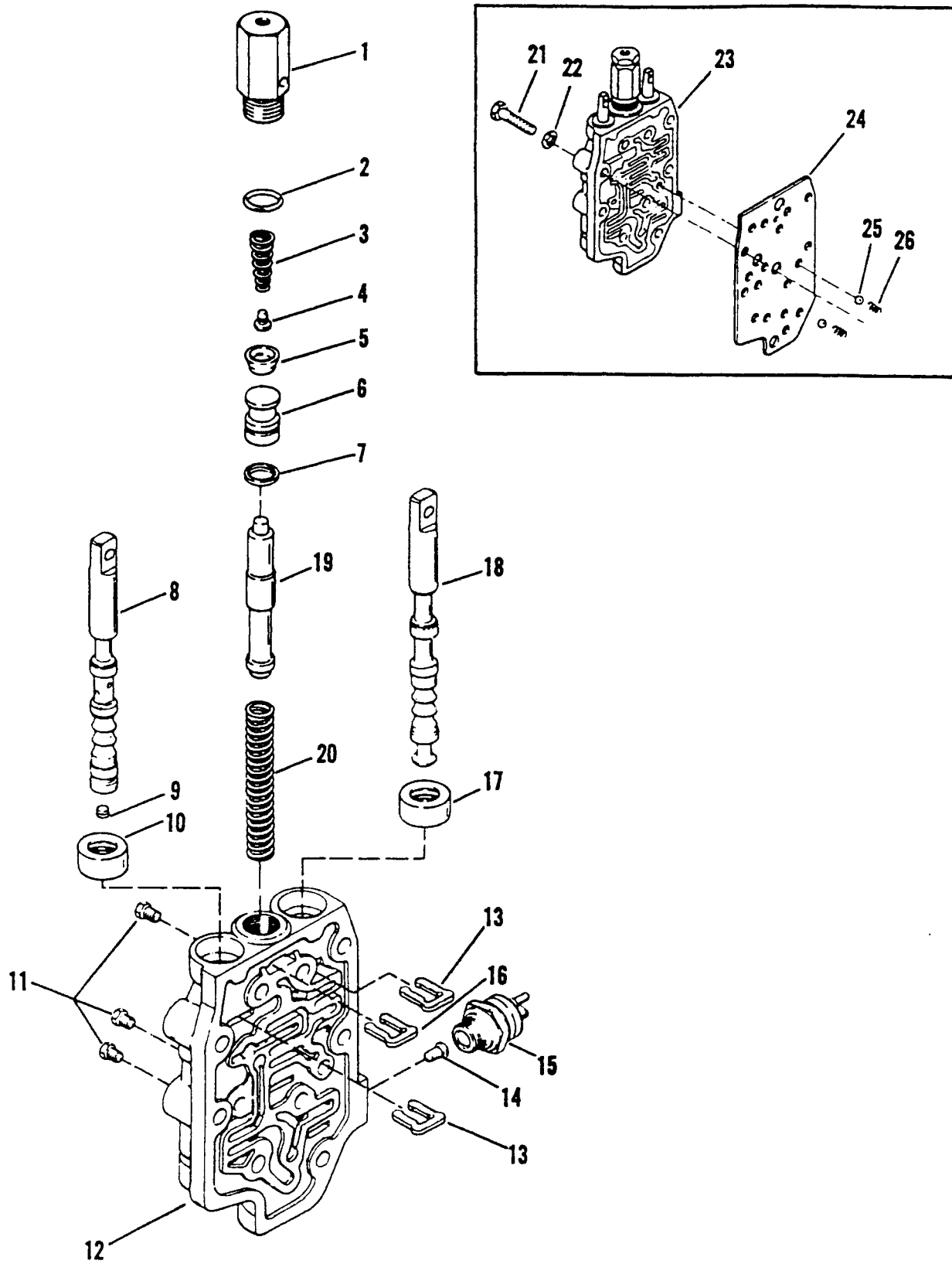
HYDRAULIC DECLUTCH
